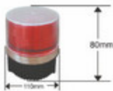
TD06-63-170 UNIVERSAL WARNING LAMP
